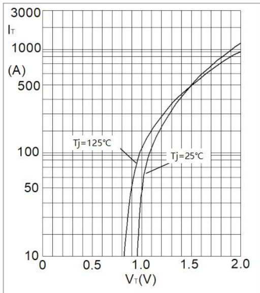
Fig4. Forward Characteristics
