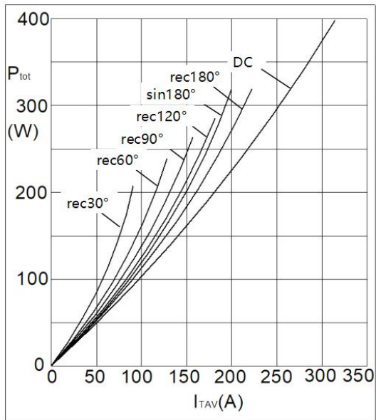
Fig2. Power Dissipation
